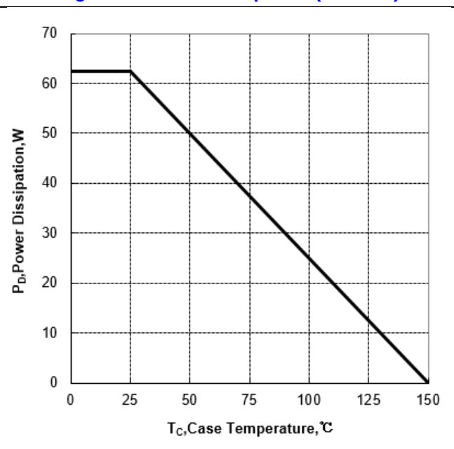
Figure 2b Power Dissipation (FullPAK)
