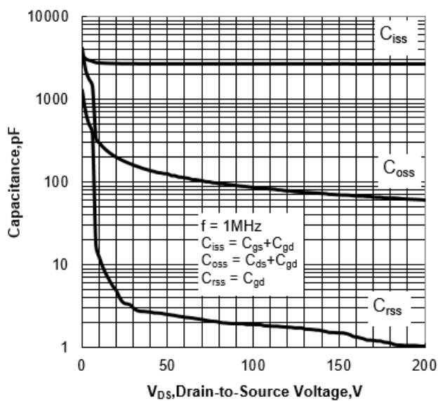
Figure 10 Capacitance Characteristics
